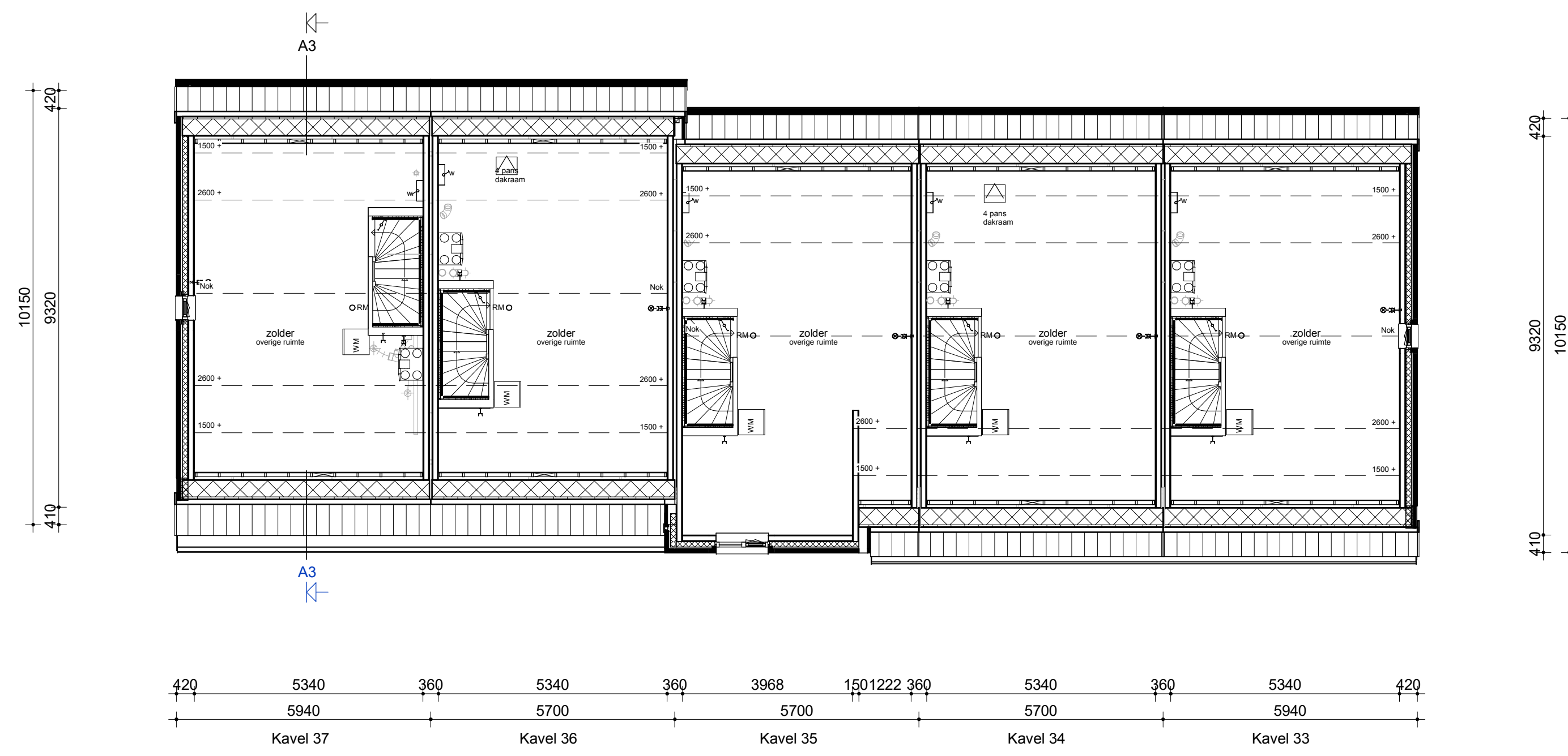
Zolder
